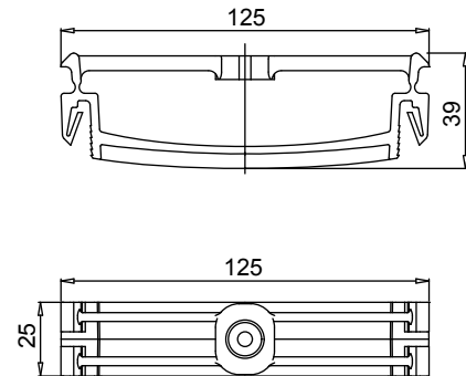
Clip Nylon
