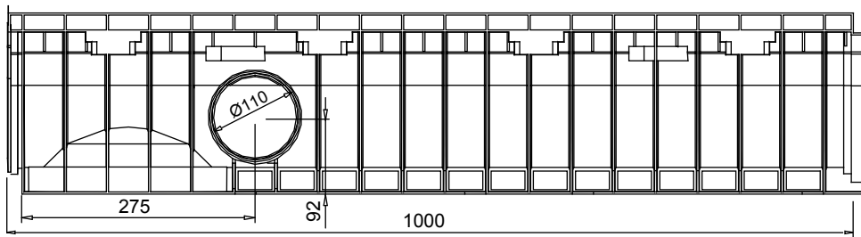
FRONTAL VIEW
